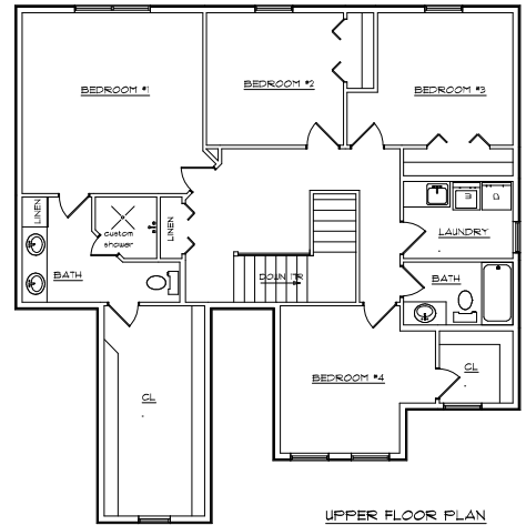
UPPER FLOOR PLAN 1311 sq.ft.
