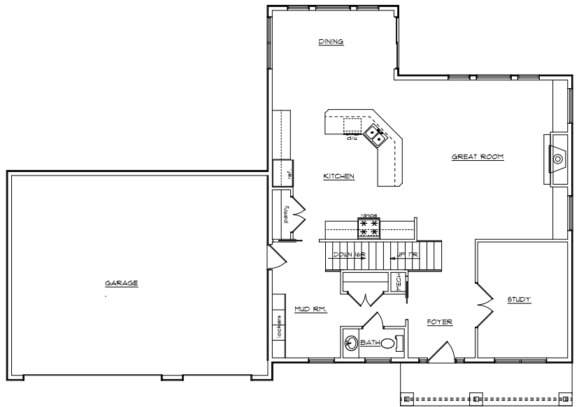
MAIN FLOOR PLAN 1278 sq.ft.
