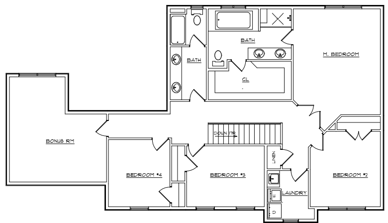
UPPER FLOOR PLAN 1584 sq.ft.
