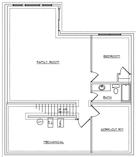
FOUNDATION PLAN 946 sq.ft. finished 352 sq.ft. mechanical
