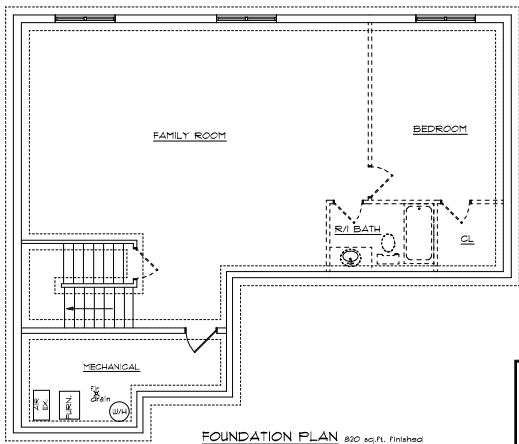
FOUNDATION PLAN 820 sq.ft. finished
