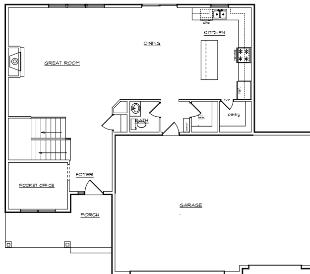
MAIN FLOOR PLAN 1142 sq.ft.
