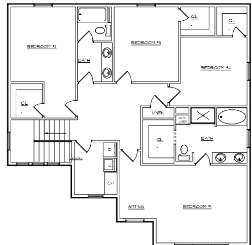
UPPER FLOOR PLAN 1373 sq.ft.
