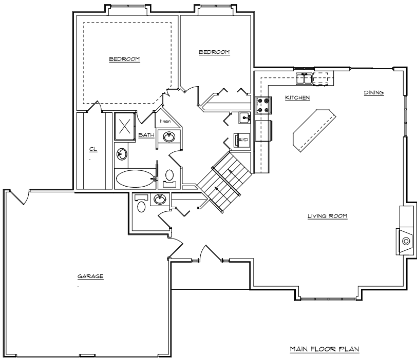
MAIN FLOOR PLAN 562 sq.ft.
