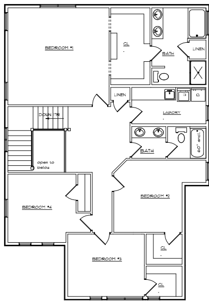
UPPER FLOOR PLAN 1342 sq.ft.
