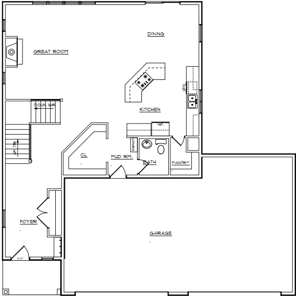
MAIN FLOOR PLAN 1160 sq.ft.
