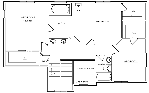
UPPER FLOOR PLAN 1094 sq./ft.
