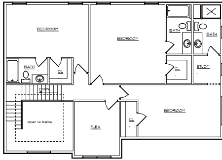
UPPER FLOOR PLAN 1246 sq.ft.
