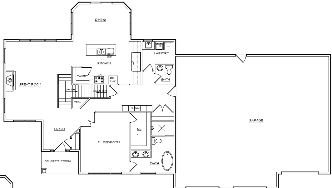
MAIN FLOOR PLAN 1612 sq.ft.
