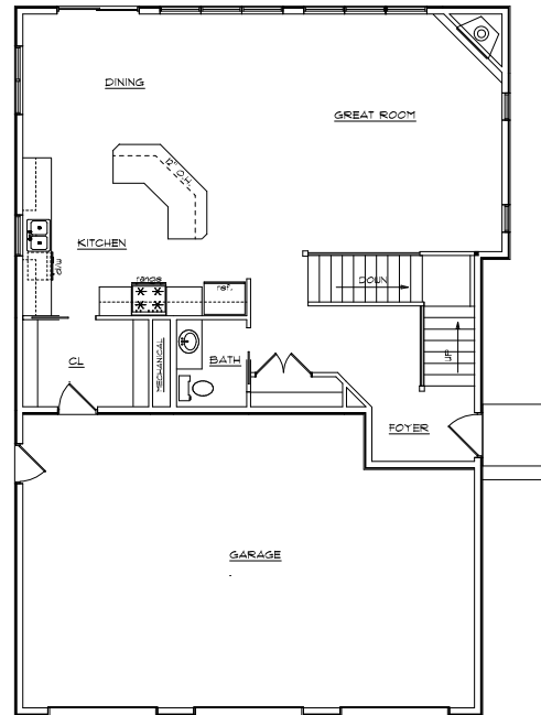
MAIN FLOOR PLAN 1080 sq.ft.
