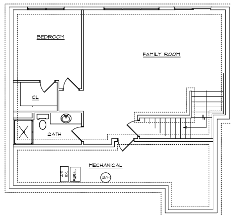
FOUNDATION PLAN 760 sq.ft. finished
