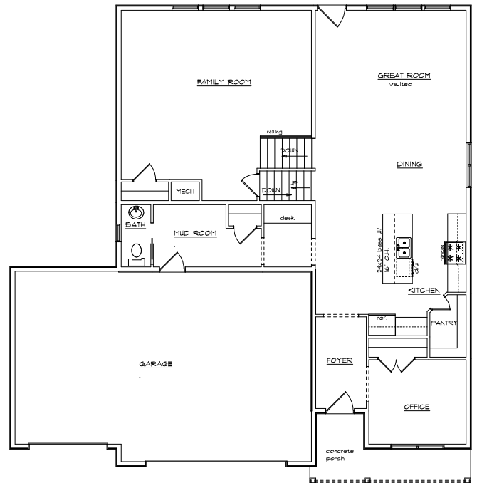
MAIN FLOOR PLAN 1536 sq.ft.
