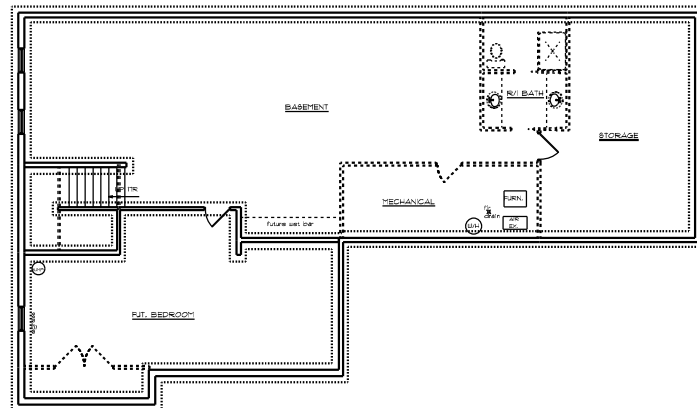
FOUNDATION PLAN
